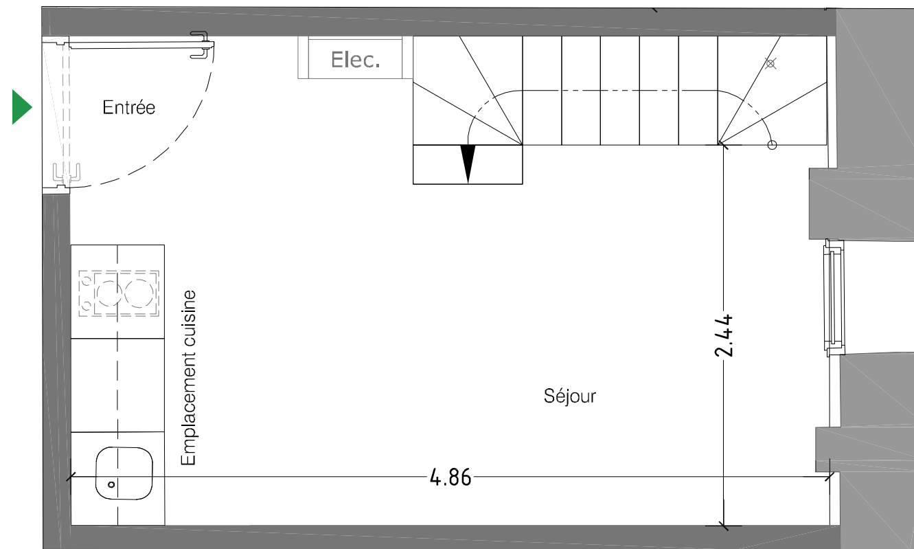
R+1
